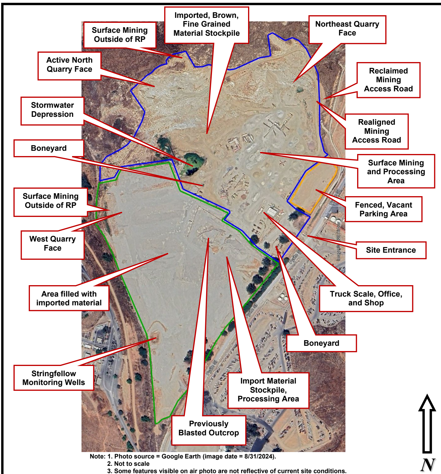
FIGURE 2 SITE LAYOUT MAP
